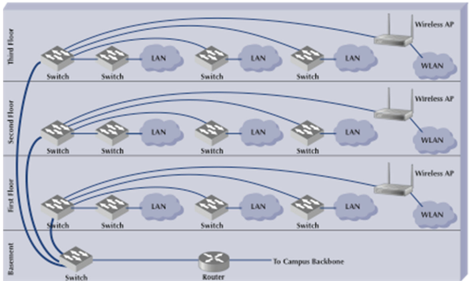
FIGURE 8-4 Switched backbones at Indiana University
